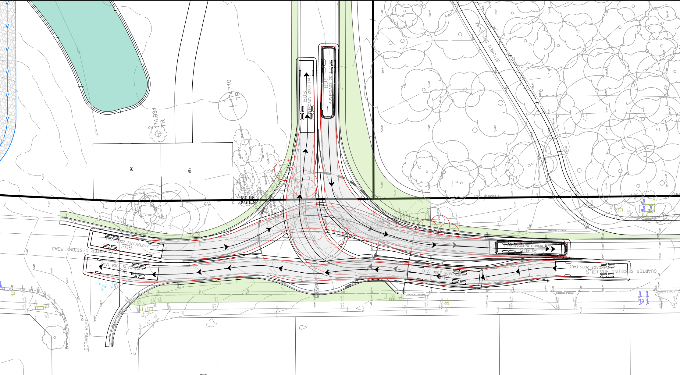
QUARTER SESSIONS ROAD & SEFTON ROAD EXTENSION ROUNDABOUT
