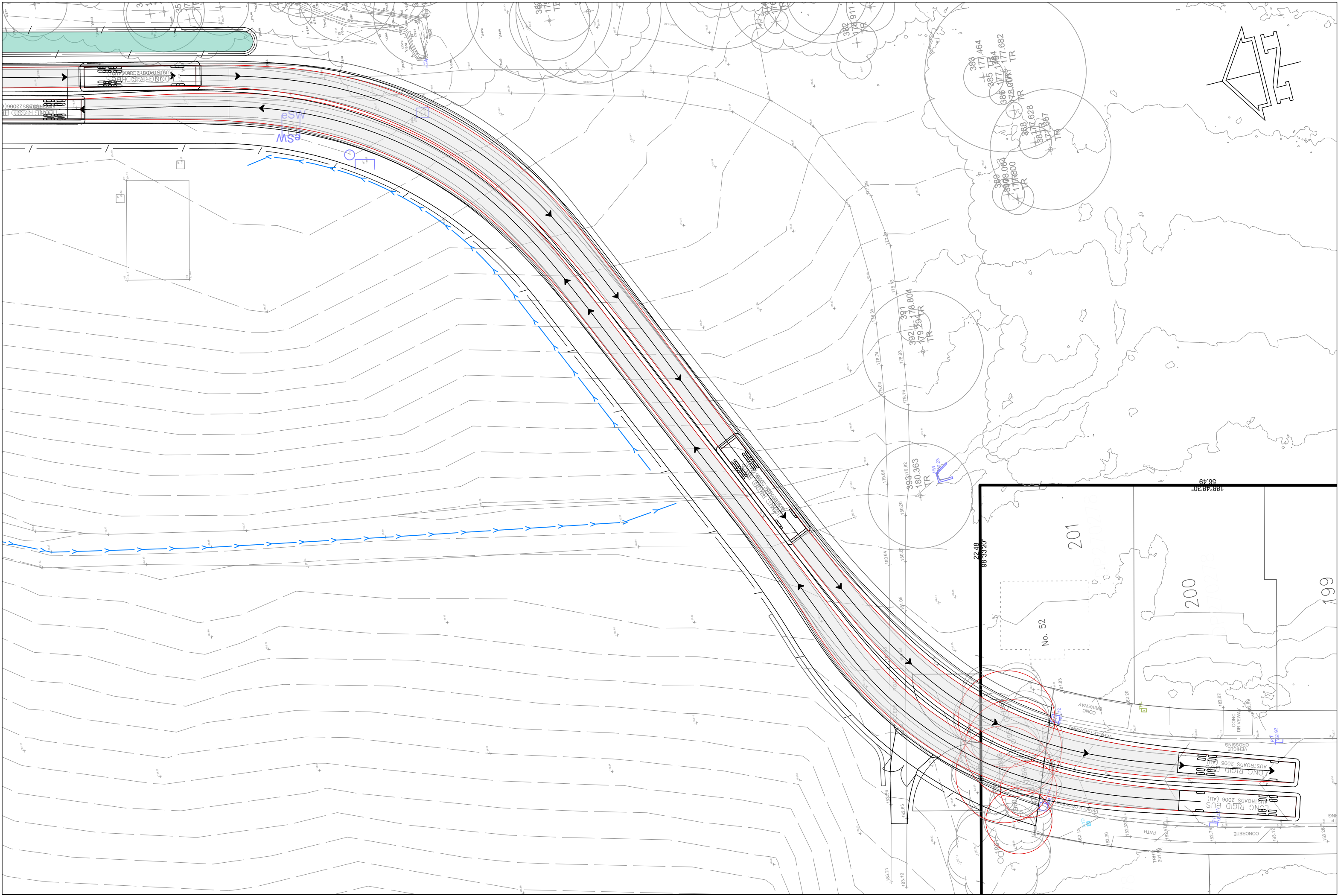
SEFTON ROAD EXTENSION - SOUTH GATE ROUNDABOUT
