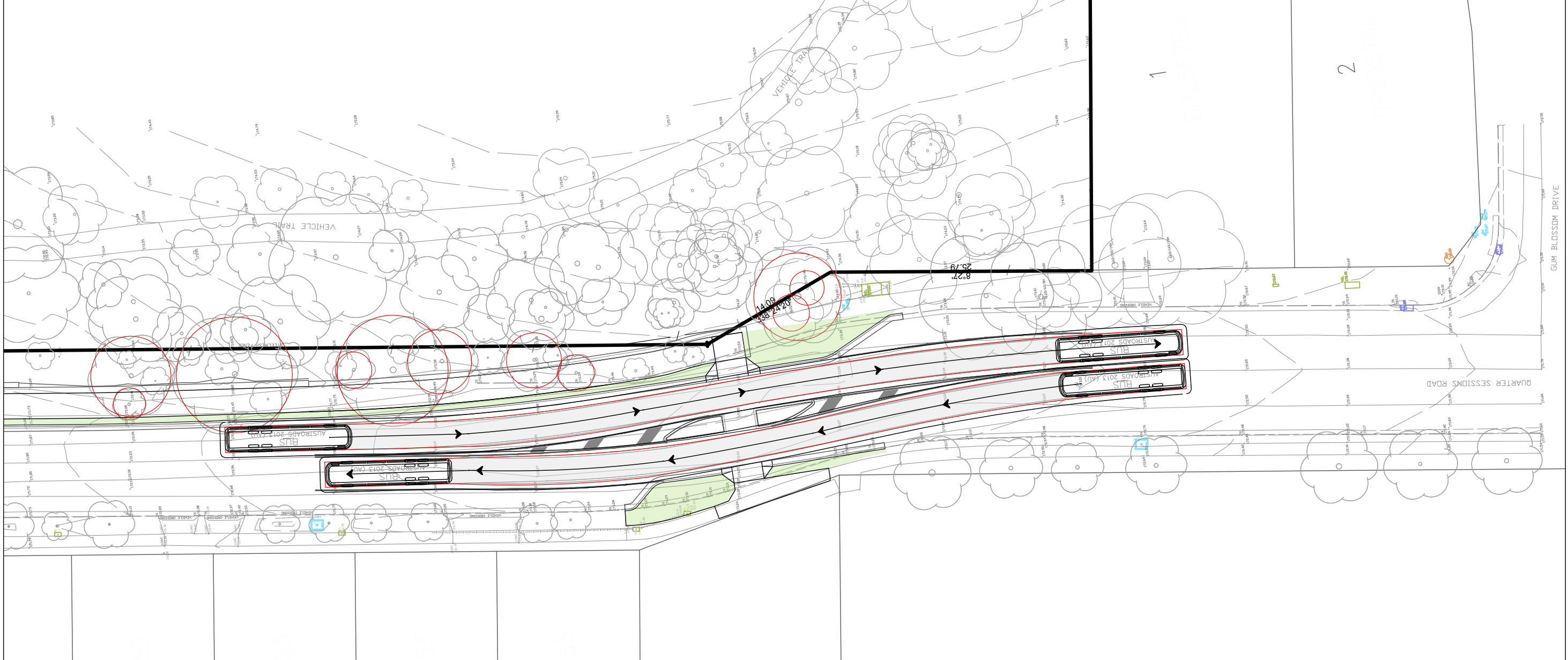
QUARTER SESSIONS ROAD - RUDDOCK PARK REFUGE ISLAND CROSSING
