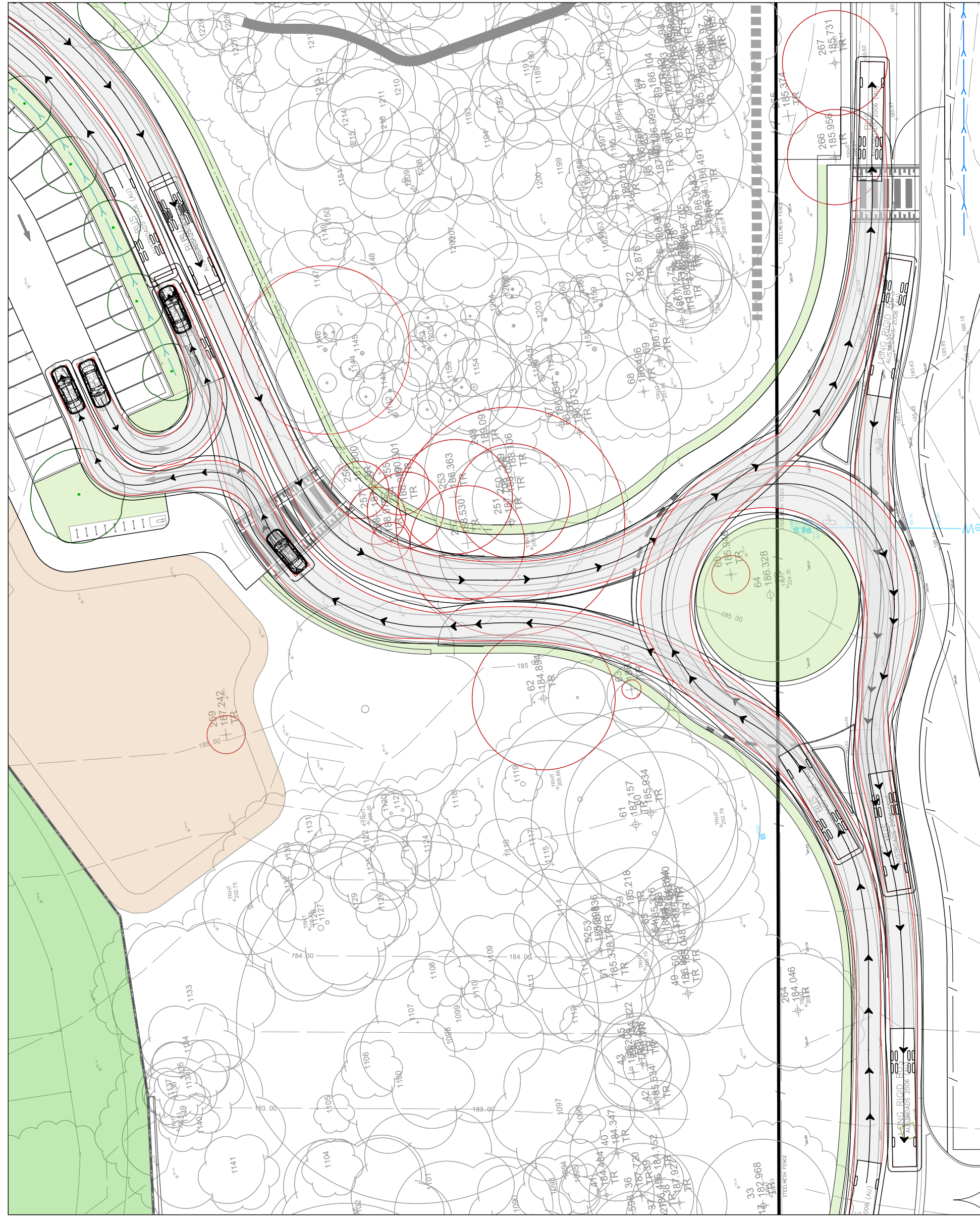
SEFTON ROAD EXTENSION - SOUTH GATE ROUNDABOUT
